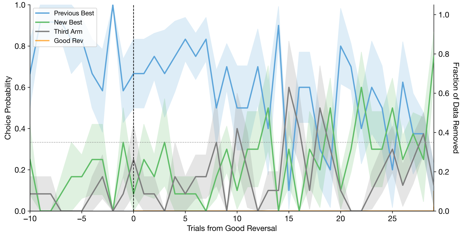
Good Reversal-Aligned Choices (mean \pm se across subjects | n=6 subjects, n=10 reversals)
